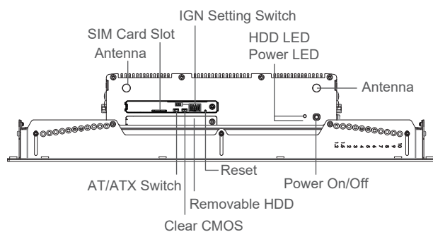
Front I/O
