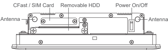
Front I/O
