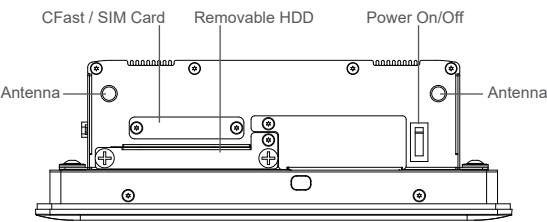
Front I/O
