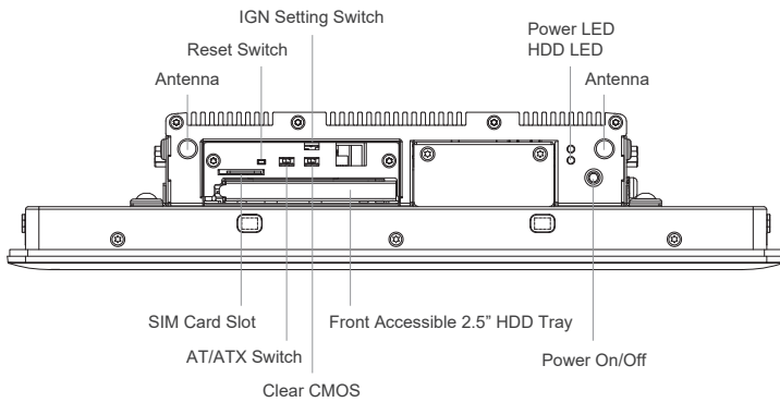
Front I/O
