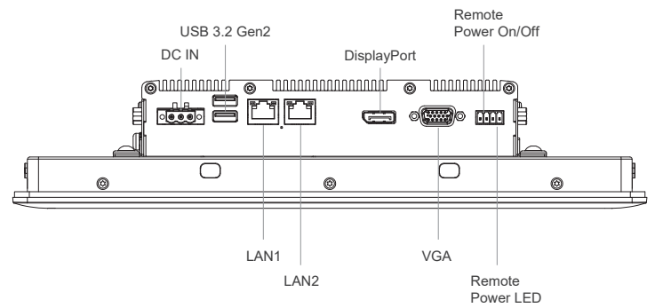
Rear I/O
