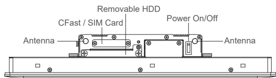
Front I/O
