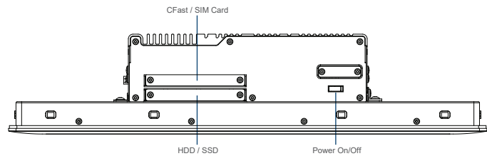
Rear I/O
