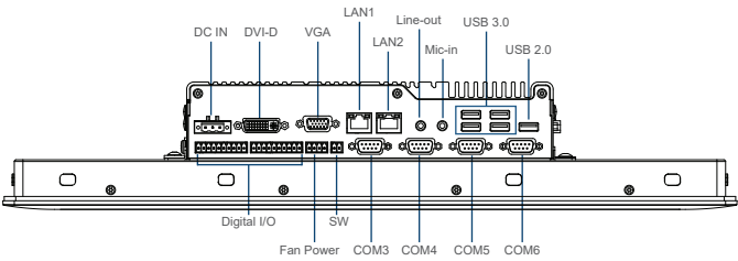
Front I/O
