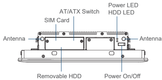
Front I/O
