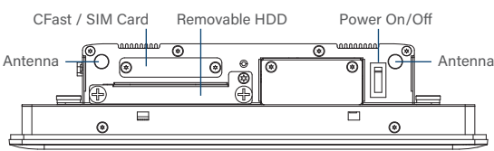
Front I/O
