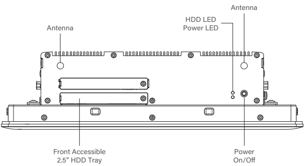
Front I/O
