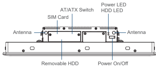
Front I/O
