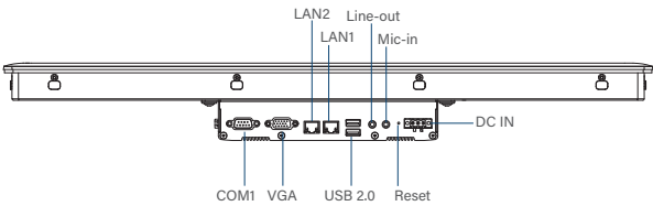
Rear I/O
