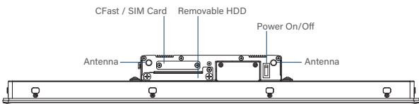
Front I/O
