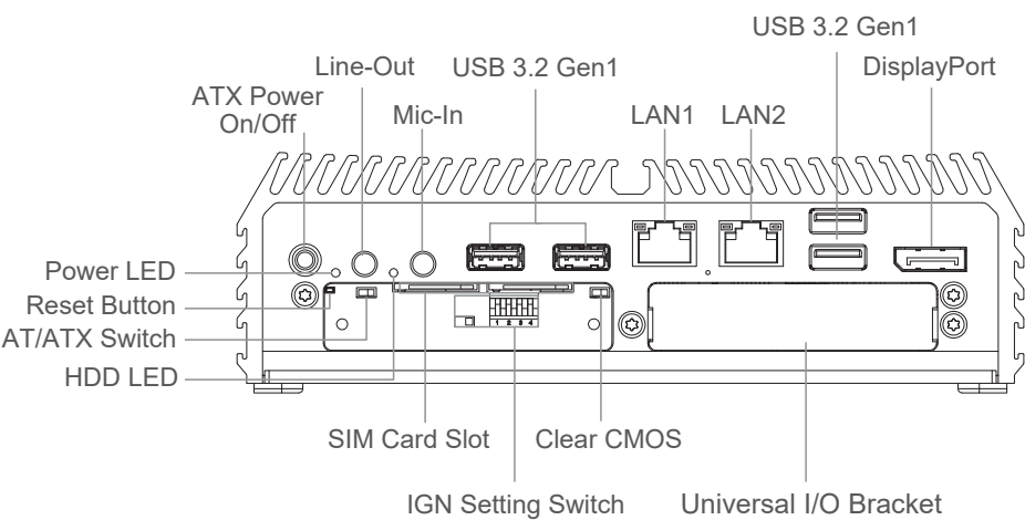
Front I/O
