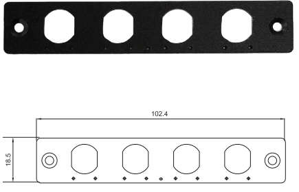
UB1310 Universal Bracket with 4x M12 Cutout Dimension (WxD): 102.4 x 18.5 mm
