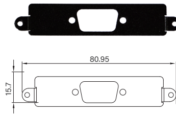
UB1116 Universal Bracket with VGA Cutout Dimension (WxD) : 80.95 x 15.7 mm
