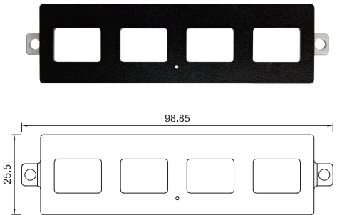
UB1412 Universal Bracket with 4x RJ45 Cutout Dimension (WxD): 98.85 x 25.5 mm
