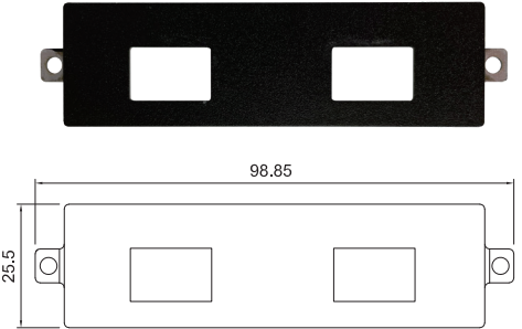
UB1428 Universal Bracket with 2x RJ45 Cutout Dimension (WxD): 98.85 x 25.5 mm
