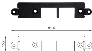
UB1129 Universal Bracket with 2x RJ45 Cutout for DC-1200 Rear Bezel Dimension (WxD) : 81.6 x 15.7 mm
