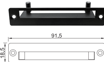
UB1618 Universal Bracket with DIO Cutout Dimension (WxD): 91.5 x 18.5 mm
