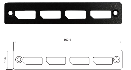
UB1329 Universal Bracket with 4x DP Cutout Dimension (WxD): 102.4 x 18.5 mm
