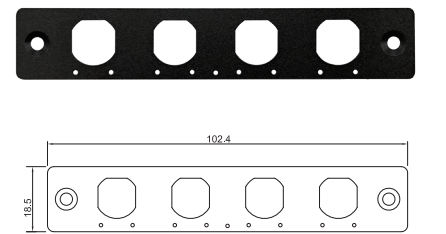
UB1330 Universal Bracket with 4x M12 X-Coded Cutout Dimension (WxD): 102.4 x 18.5 mm
