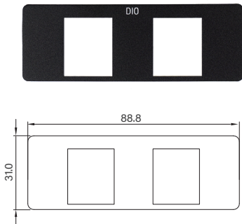
UB1018 Universal Bracket with DIO Cutout Dimension (WxD) : 88.8 x 31.0 mm
