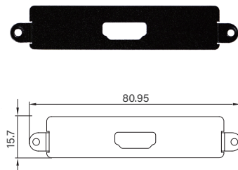
UB1108 Universal Bracket with HDMI Cutout Dimension (WxD) : 80.95 x 15.7 mm
