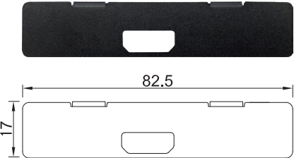
UB1508 Universal Bracket with HDMI Cutout Dimension (WxD): 82.5 x 17 mm
