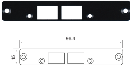
UB0411 Universal Bracket with 2x RJ45 Cutout Dimension (WxD) : 96.4 x 15 mm
