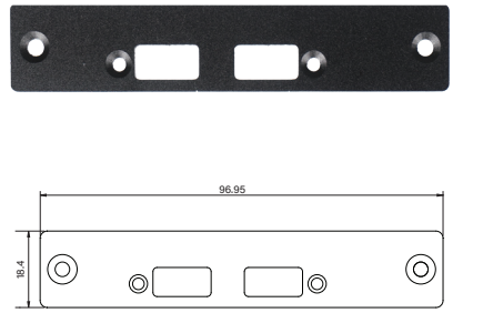
UB1314 Universal Bracket with 2x USB Cutout Dimension (WxD): 96.95 x 18.4 mm
