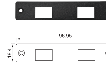
UB1728 Universal Bracket with 2x RJ45 Cutout for CMI-10GLAN Expansion Dimension(WxD): 96.95 x 18.4mm
