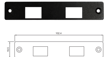
UB1328 Universal Bracket with 2x RJ45 Cutout Dimension (WxD): 102.4 x 18.5 mm
