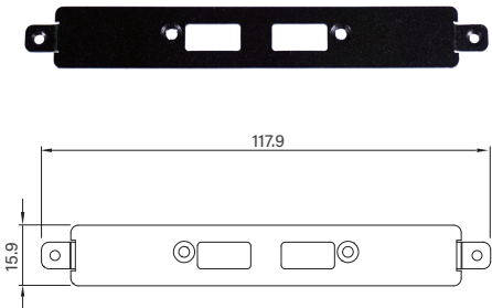
UB1214 Universal Bracket with 2x USB Cutout Dimension (WxD) : 117.9 x 15.9 mm
