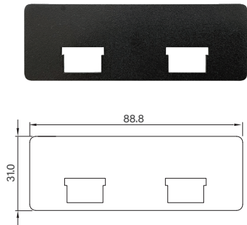
UB1028 Universal Bracket with 2x RJ45 Cutout Dimension (WxD) : 88.8 x 31 mm
