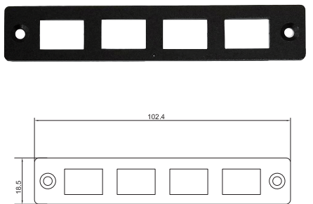
UB1312 Universal Bracket with 4x RJ45 Cutout Dimension (WxD): 102.4 x 18.5 mm
