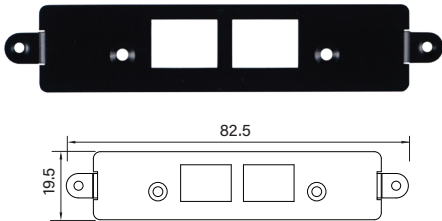
UB0711 Universal Bracket with 2x RJ45 Cutout Dimension (WxD) : 82.5 x 19.5 mm
