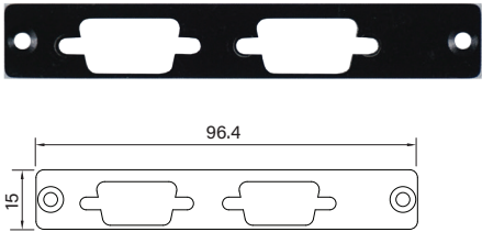
UB0403 Universal Bracket with 2x DB9 Cutout Dimension (WxD) : 96.4 x 15 mm
