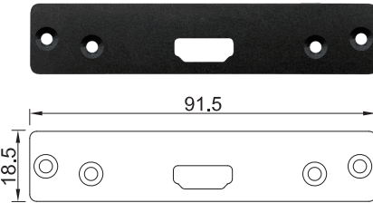
UB1608 Universal Bracket with HDMI Cutout Dimension (WxD): 91.5 x 18.5 mm
