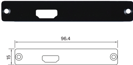
UB0408 Universal Bracket with HDMI Cutout Dimension (WxD) : 96.4 x 15 mm
