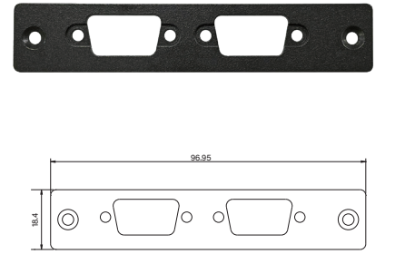
UB1303 Universal Bracket with 2x DB9 Cutout Dimension (WxD): 96.95 x 18.4 mm
