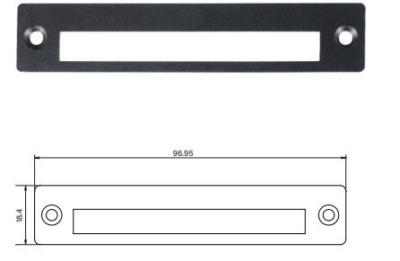
UB1318 Universal Bracket with DIO Cutout Dimension (WxD): 96.95 x 18.4 mm
