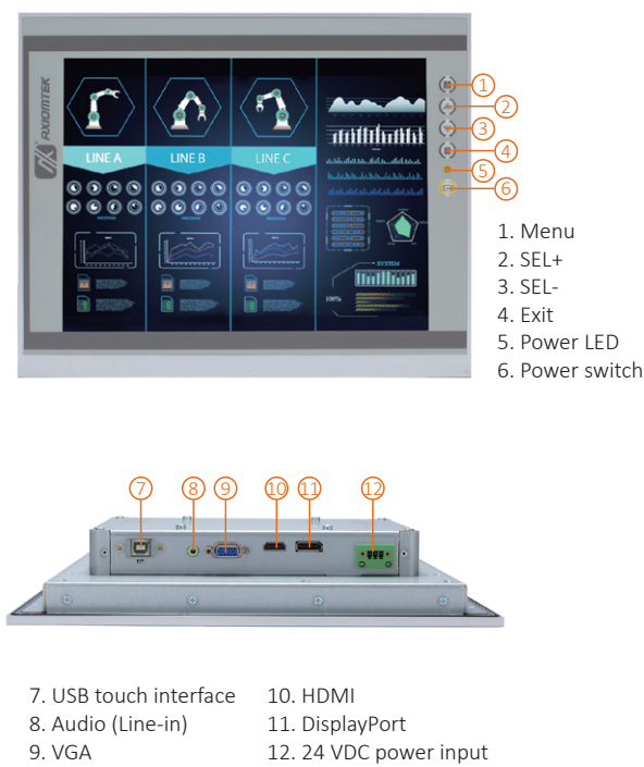
▲ Ultra-slim mechanism design
